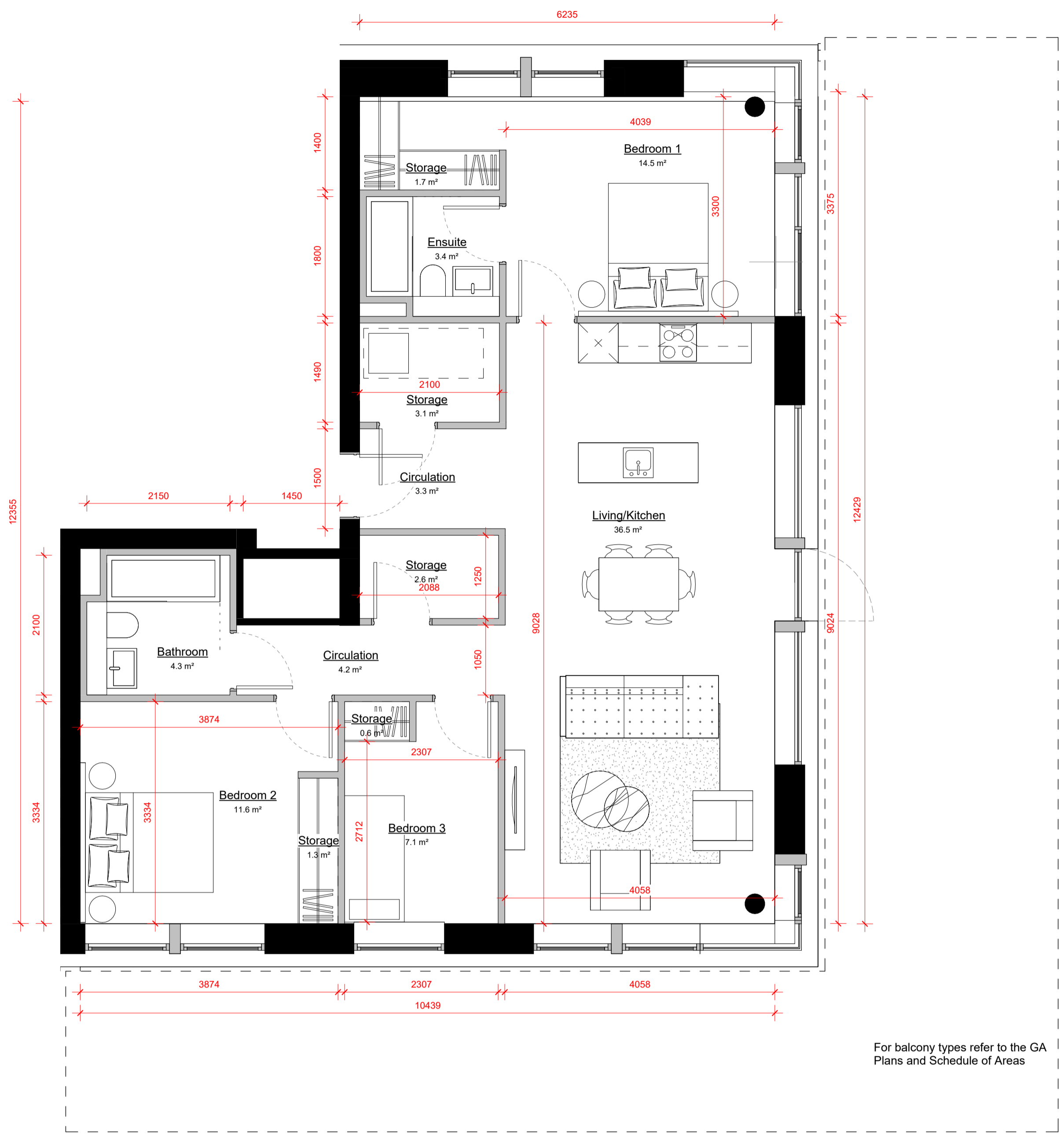
Apartment Type C.8.0 1 : 50
